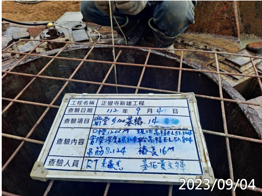
齋堂全套管基樁深度查驗
